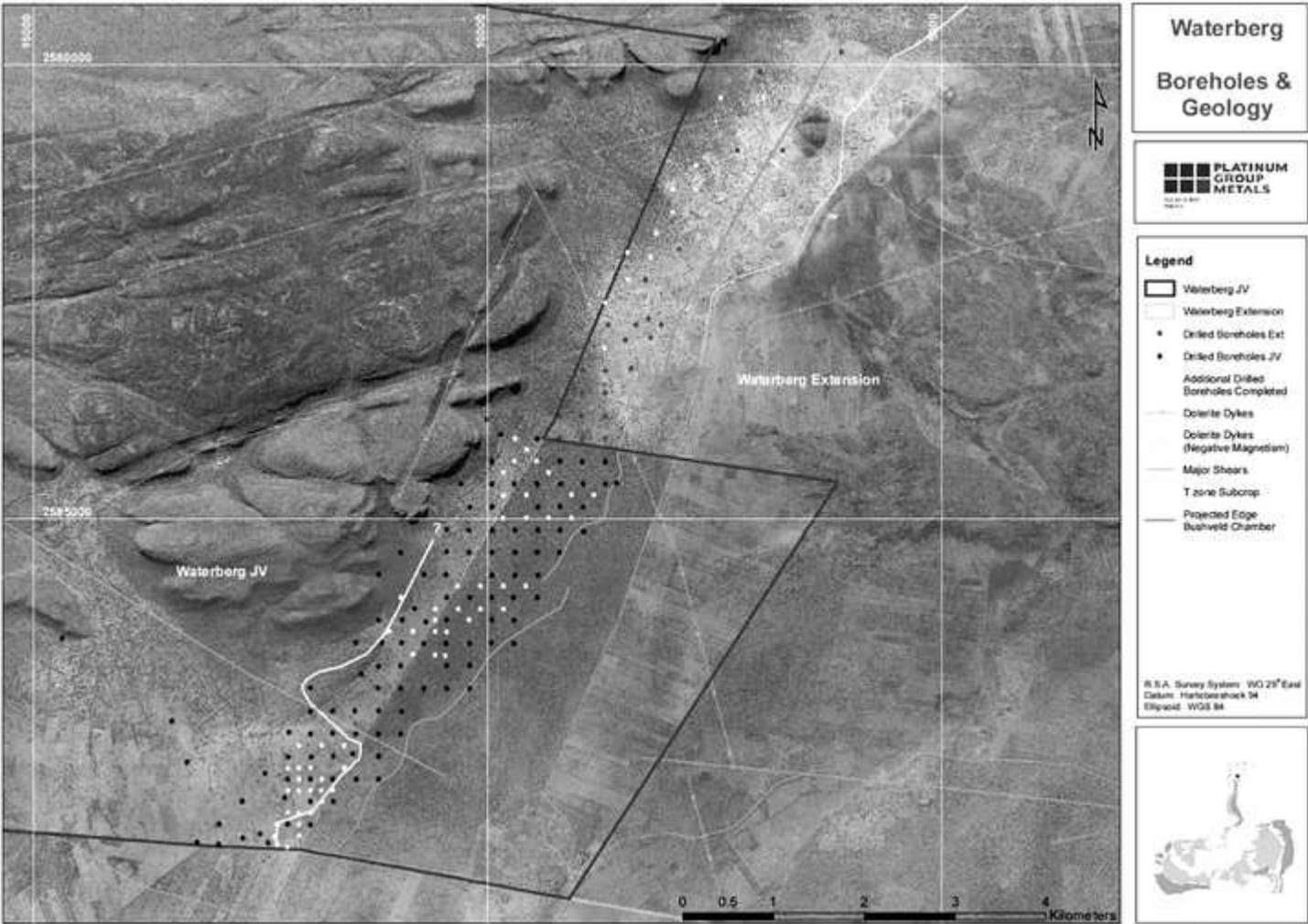
Figure 1.5_1 Borehole Location and Geology of the Waterberg JV and Extension Projects
